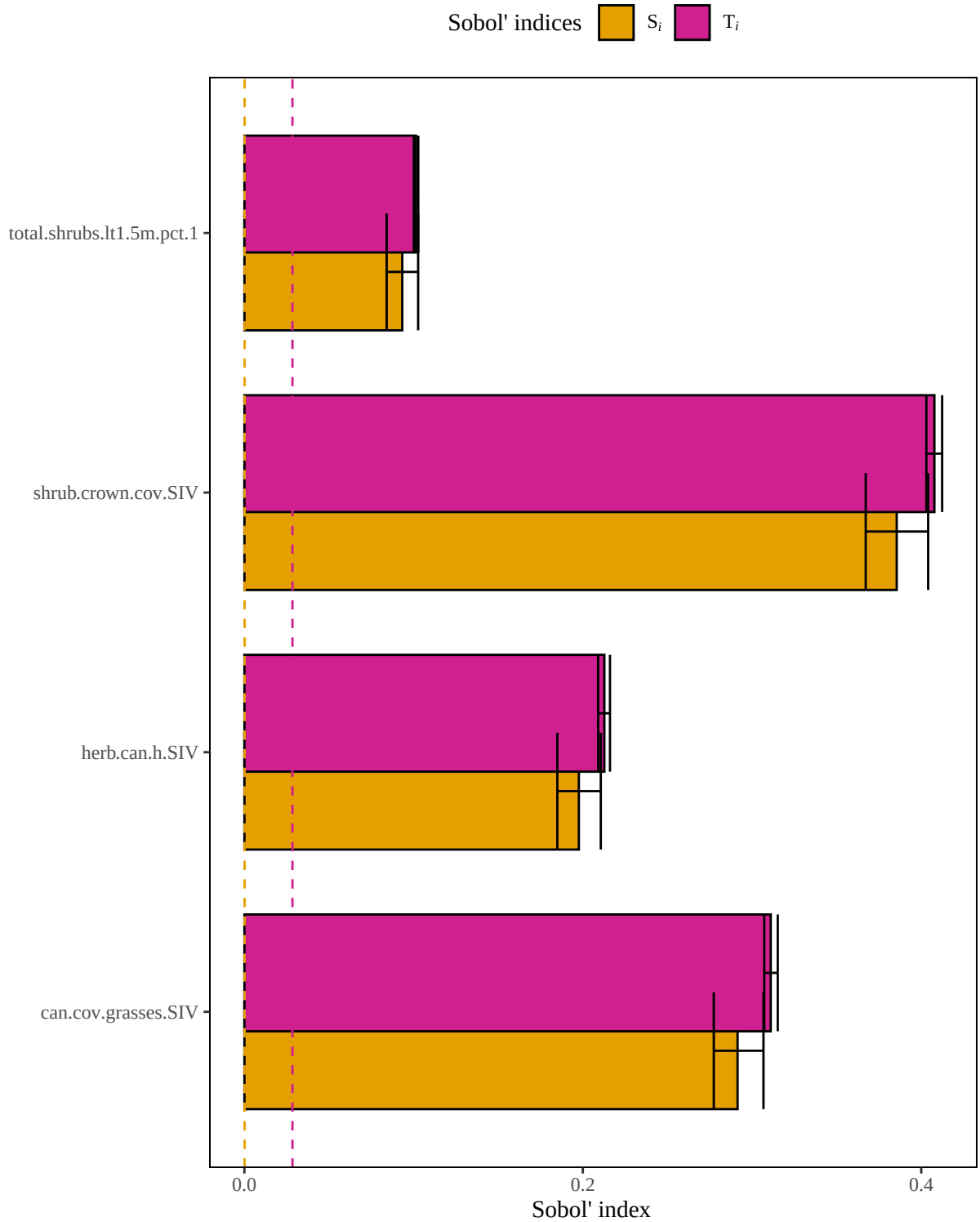
Figure 5. Results of a sensitivity analysis for the fieldsparrow model based on a geometric mean structure. Dashed lines represent baseline numerical approximation error for S_i and T_i ( i.e. , dummy variables).
